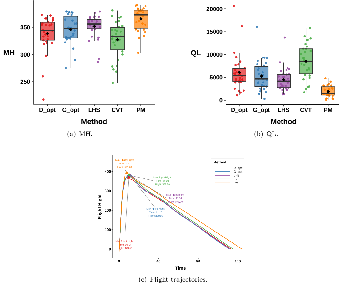
Figure 9. Optimization results of different methods: (a) MH; (b) QL; (c) Flight trajectories.
